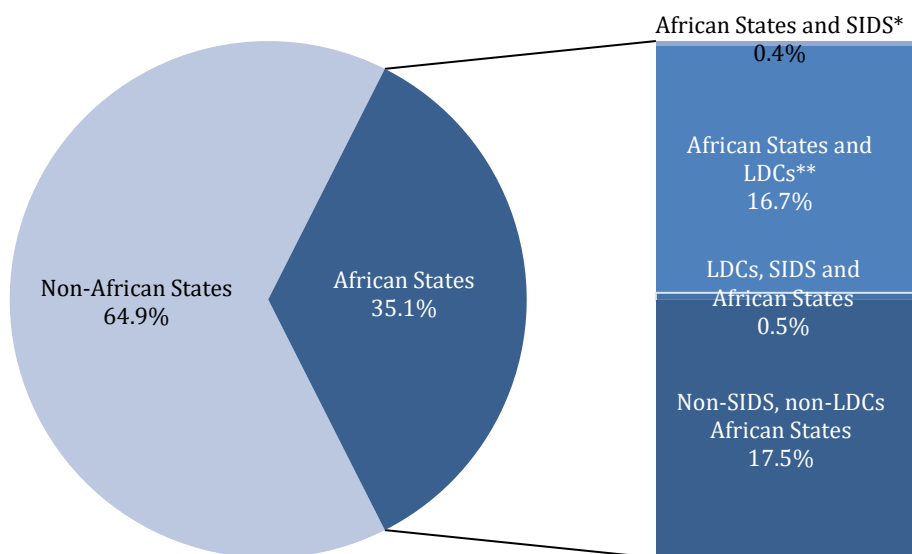
Figure 3.3: African States distribution of the GCF requested funding amount
