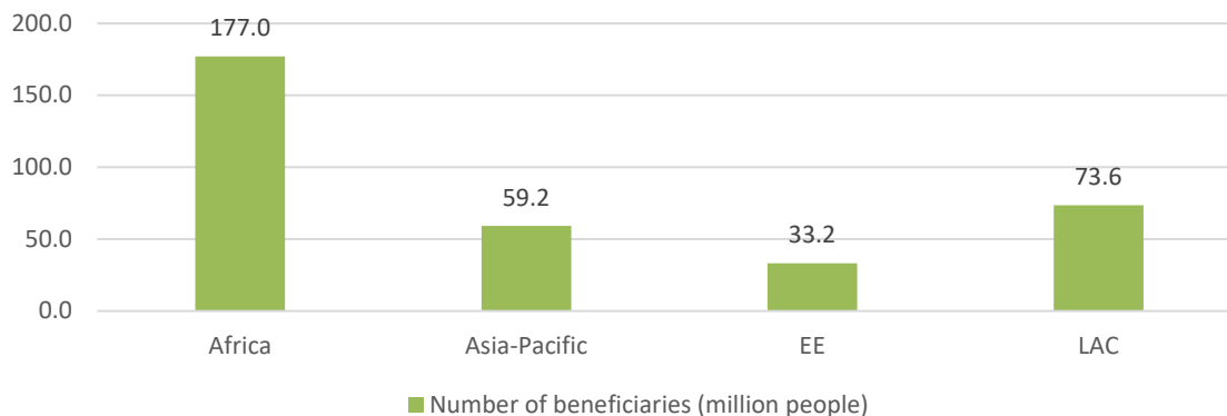
Figure 8: Estimated adaptation impact potential by region (total: 342.9 million people) a
