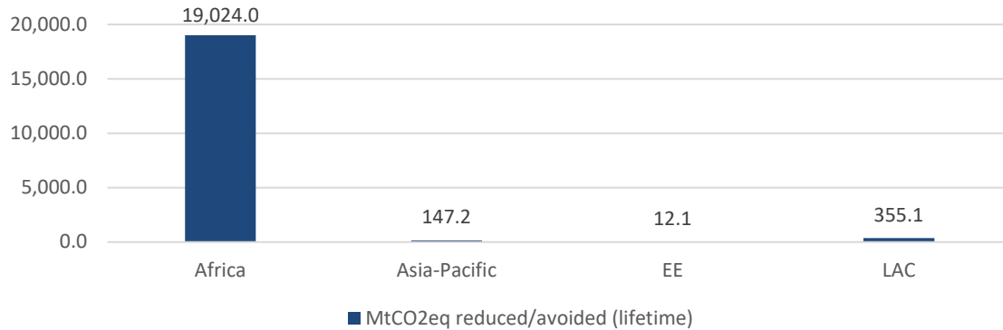
Figure 7: Estimated mitigation impact potential by region (total: 19,538.4 MtCO 2 eq) a
