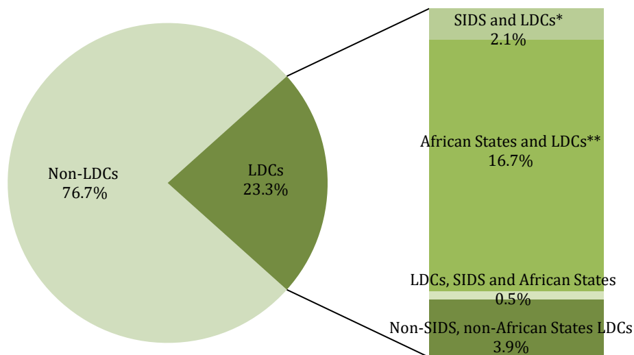
Figure 3.1: Least developed countries distribution of the GCF requested funding amount
