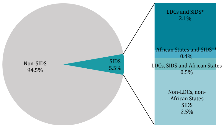
Figure 3.2: Small island developing States distribution of the GCF requested funding amount
